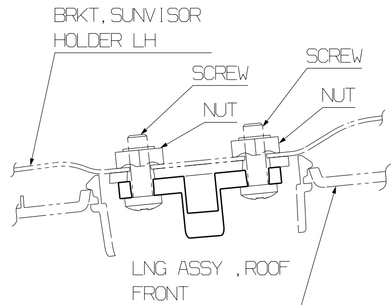
SECTION AA (1:1)
