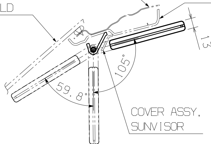
SECTION BB (1:3)
