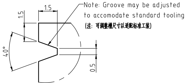
Detail A (3:1)
