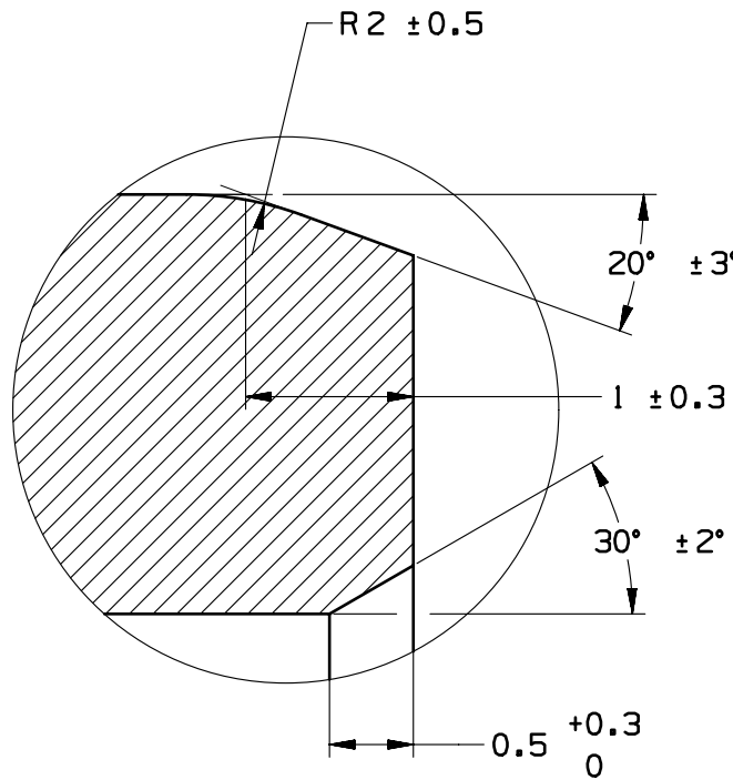
DETAIL D SCALE 20:1
