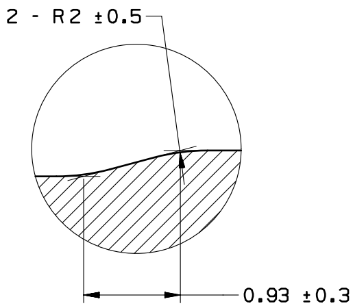
DETAIL C SCALE 20:1
